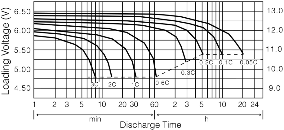
Discharge Characteristics 77°F (25°C)
